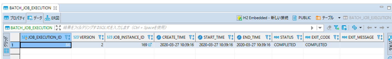
図 76. Show BATCH_JOB_EXECUTION
