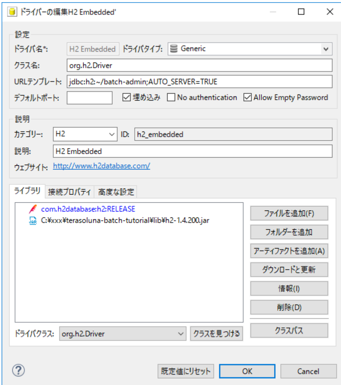
図 64. Edit Driver
