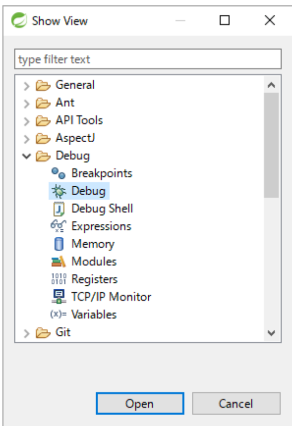
図 72. Show View
